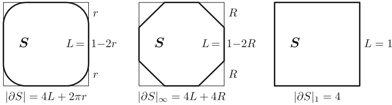
Fig. 1 The minimum cuts \partial S for \ell^2 , \ell^1 , and \ell^\infty constraints on v(x, y)
